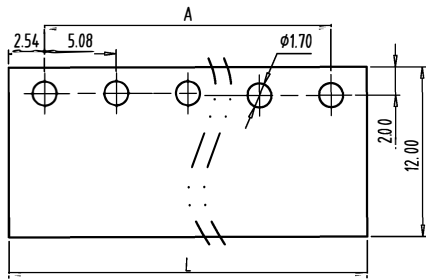
PCB LAYOUT S=2.5:1
