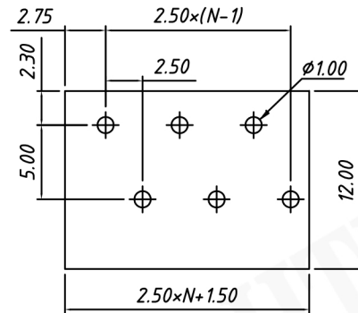
A type PCB LAYOUT
