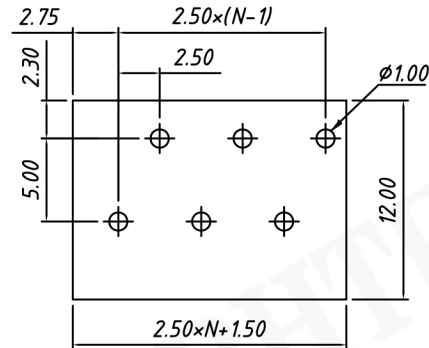
B type PCB LAYOUT
