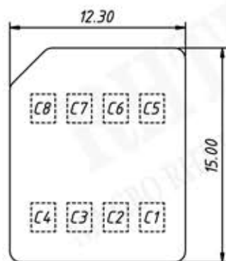
MICRO-SIM CARD DIM.(REF)
