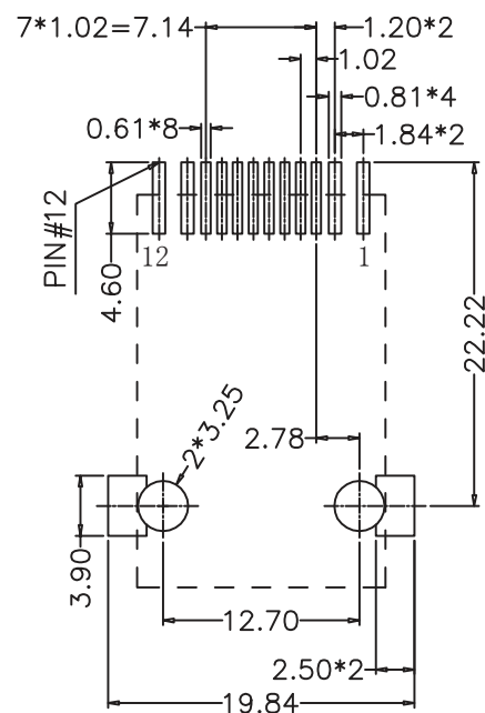
RECOMMENDED PCB LAYOUT VIEWED FROM COMPONENT SIDE
