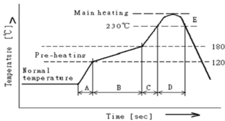
Temperature Profile
