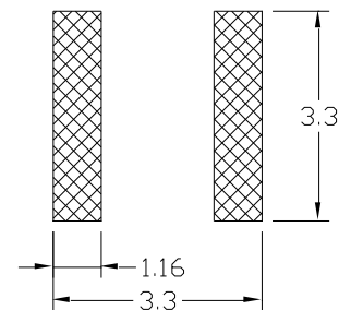
PCB PATTERN
