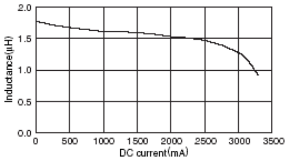
SDS5014M-1R5M-LF
