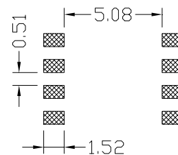
PCB PATTERN
