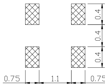
PCB PATTERN
