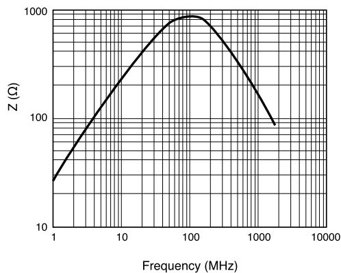
Impedance Characteristics
