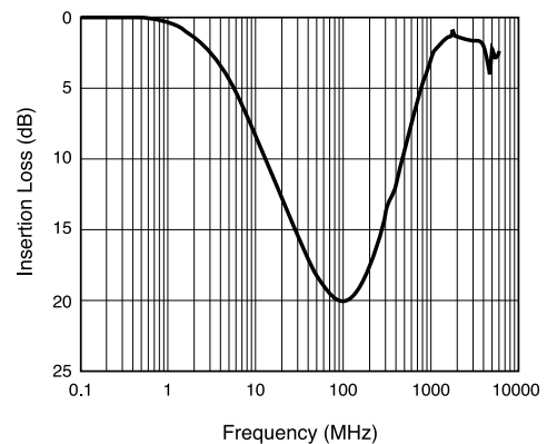
Insertion Loss Characteristics
